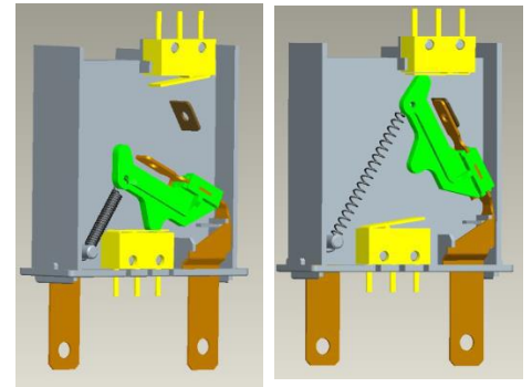
F34V internal structure
