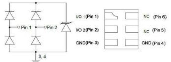
PIN Schematic
