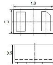
Package Dimensions
