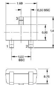
SOT-523 outline
