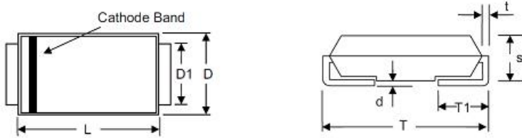
SMB/DO-214AA
